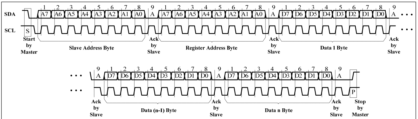
Figure 6 Writing to IS32FL3237 (Automatic Address Increment)
