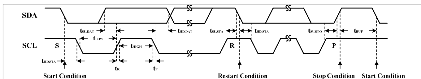
Figure 3 Interface Timing
