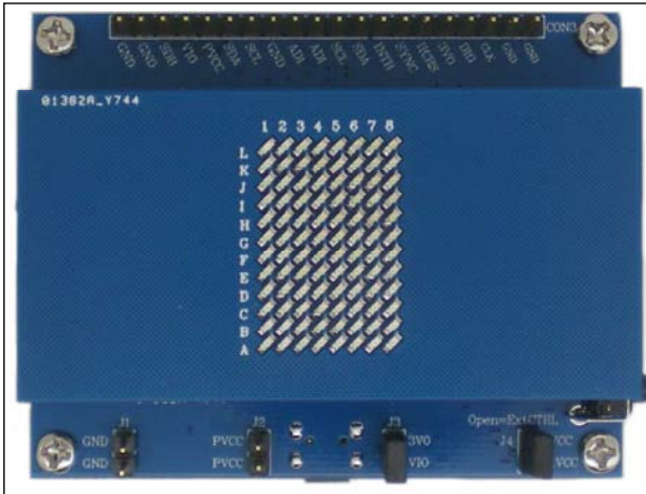
Figure 1: Photo of IS31FL3736A Evaluation Board
